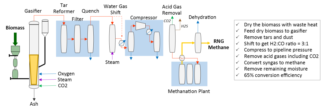
Figure 3. Thermal Gasification Production Pathway.
